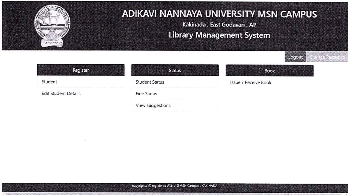
Fig. 3 : Staff dashboard
