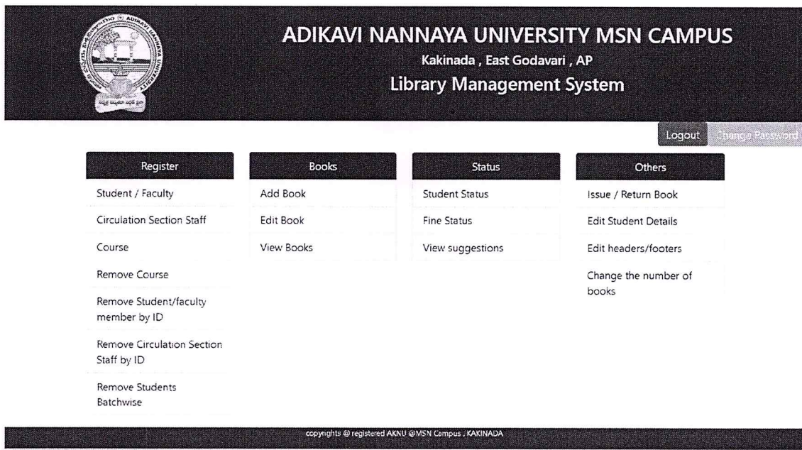
Fig. 2 : Admin dashboard
