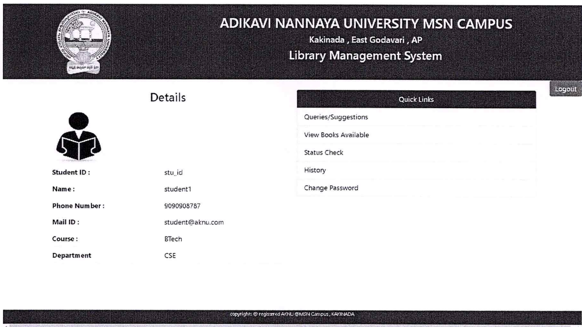
Fig. 4 : Member dashboard
